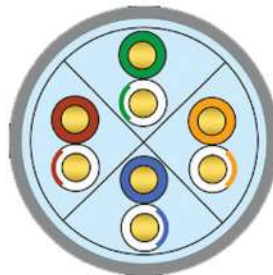
Molex PowerCAT6 UTP
